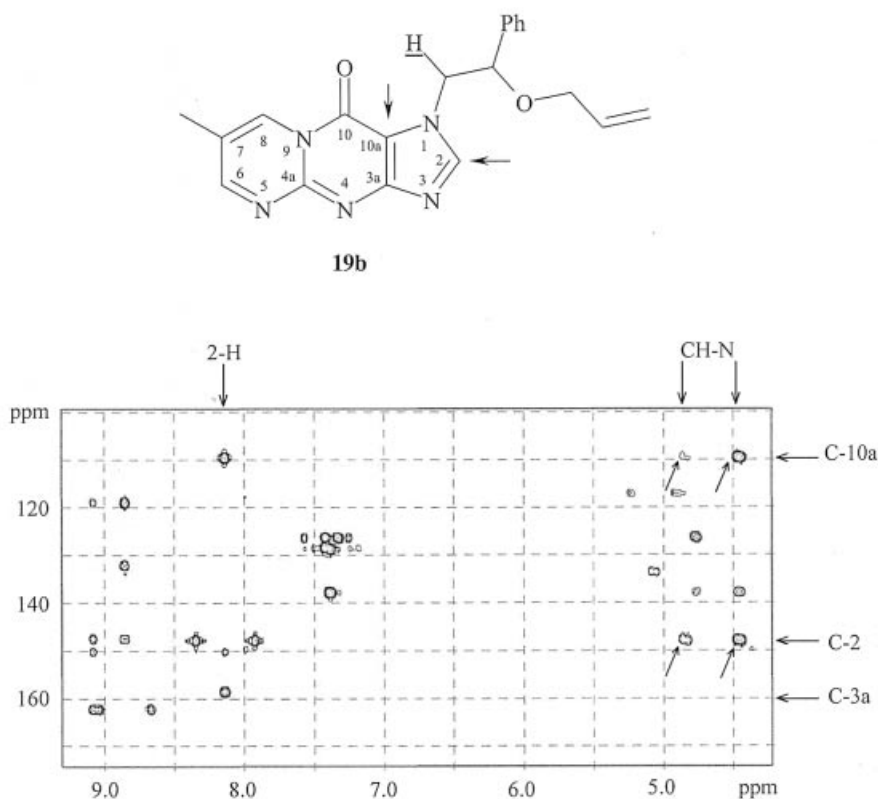
Figure 1. HMBC spectrum of 19b ; cross-peaks between \text{NCH}_2 signals and both C-2 and C-10a are highlighted, indicating that the corresponding atoms are separated by three bonds
