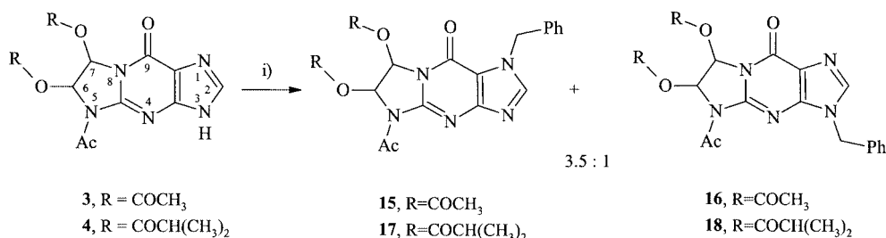
Scheme 3. Alkylation of imidazopurines 3 and 4 by reaction with benzyl bromide: i) K_2CO_3 /DMF, room temperature
