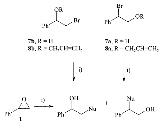
Scheme 1. Synthetic equivalents of styrene 7,8-oxide: i) \text{Nu}^- , for allyl-protected compounds 7b and 8b followed by deallylation [18]
