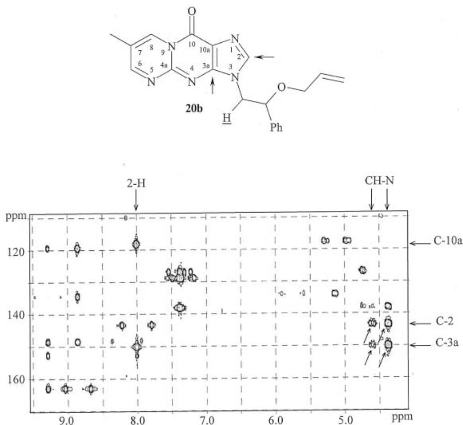
Figure 2. HMBC spectrum of 20b ; cross-peaks between \text{NCH}_2 signals and both C-2 and C-3a are highlighted, indicating that the corresponding atoms are separated by three bonds
