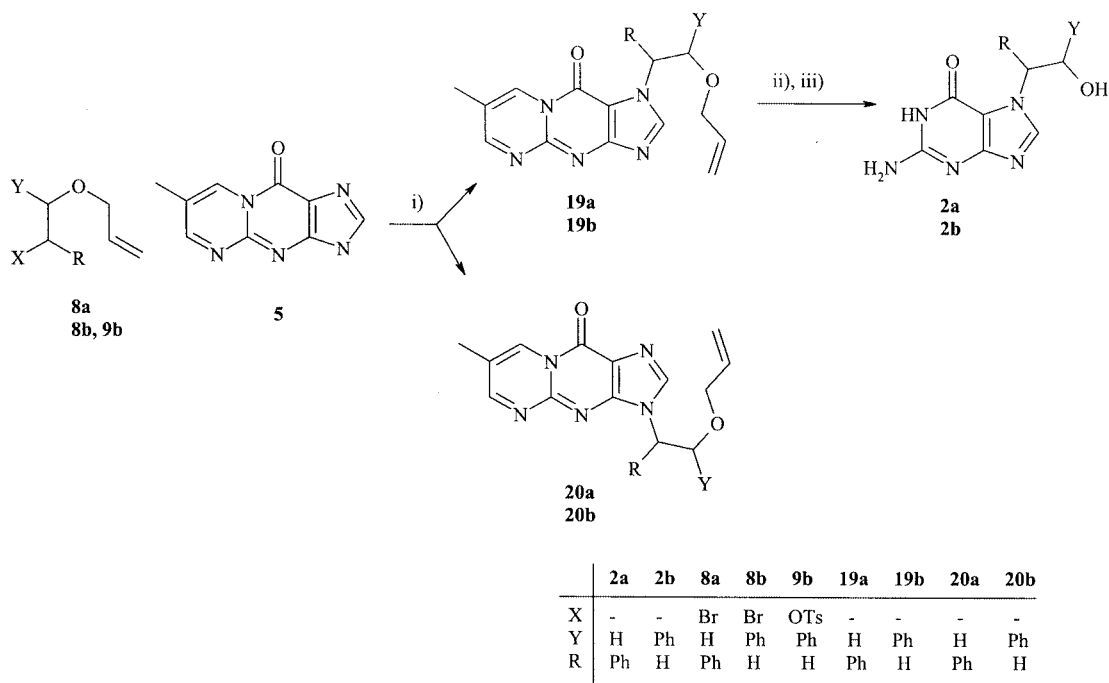
Scheme 4. Alkylation of pyrimidopurine: i) NaH or K 2 CO 3 in DMF, 60 °C, overnight; ii) aqueous NaOH, reflux, 4–6 h; iii) PMHS, [Pd(PPh 3 ) 4 ], ZnCl 2 in DMF [18]
